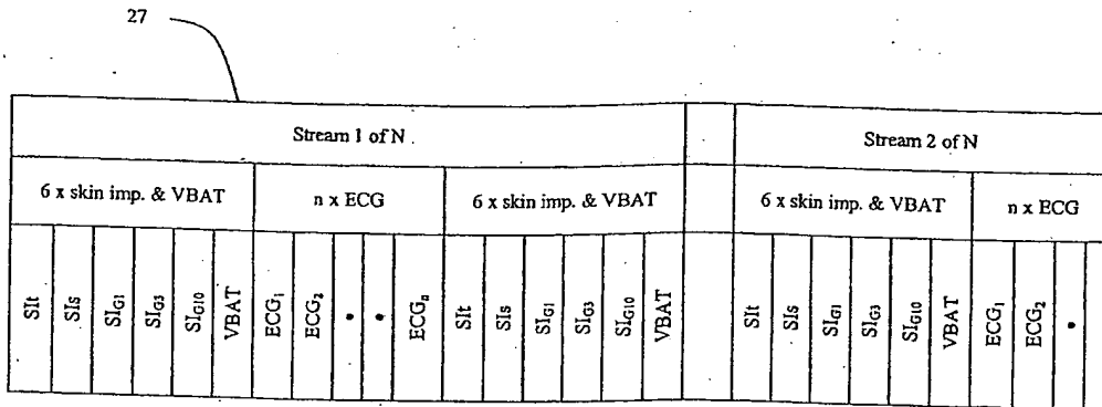
Figure 5c: Transmitter data sequence stream
